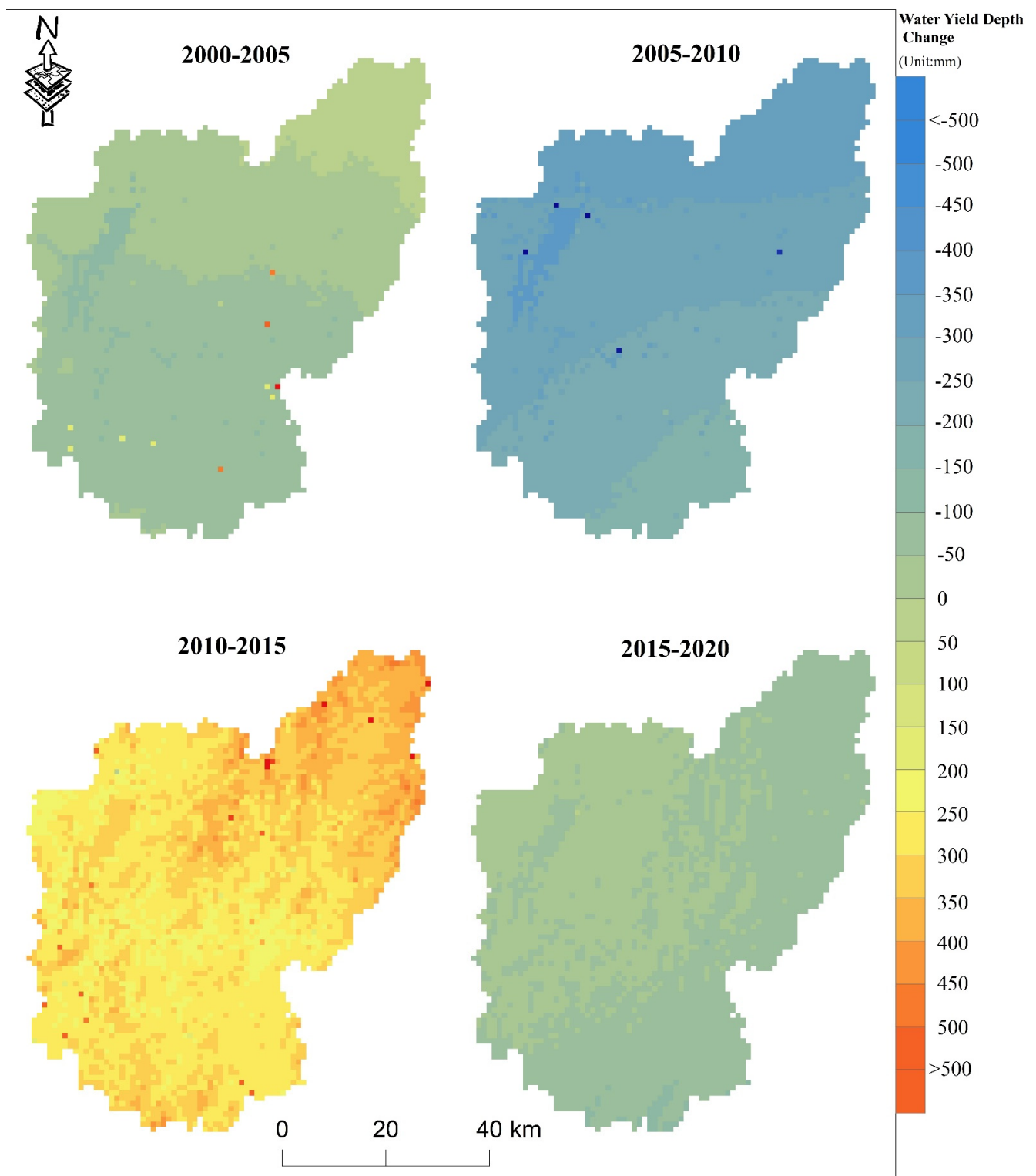
Figure 5. Spatial distribution of water production changes in the Dongjiang Lake Basin.
